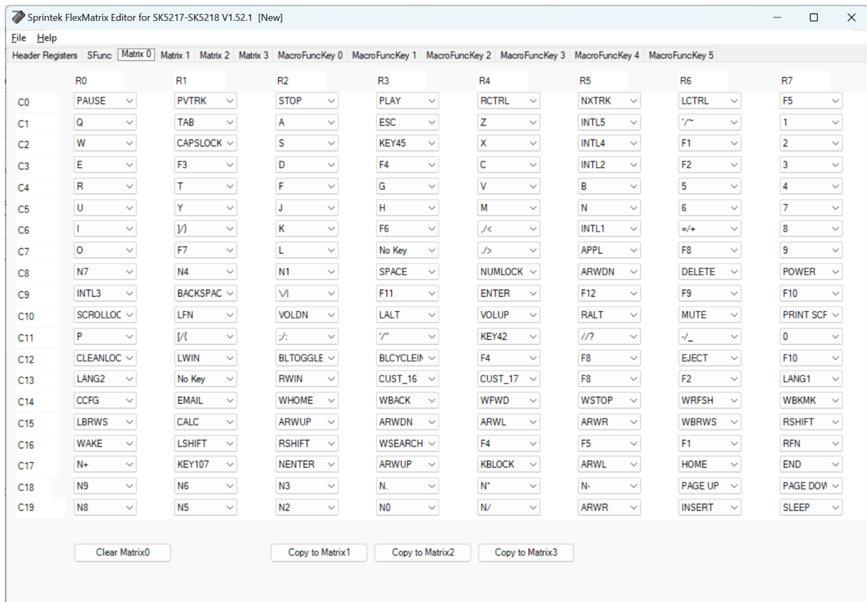
Screen snapshot of FlexMatrix™ Editor
