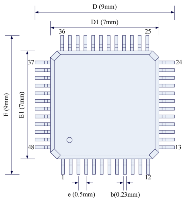
SK5301-LP Drawing
